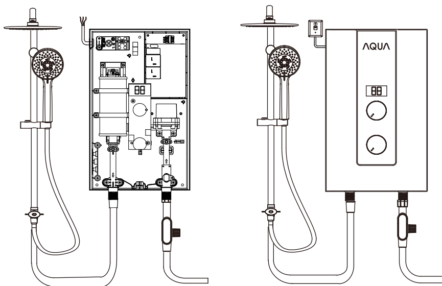
Top-spraying type
